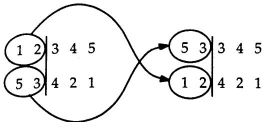
Figure 1. One-point crossover.
