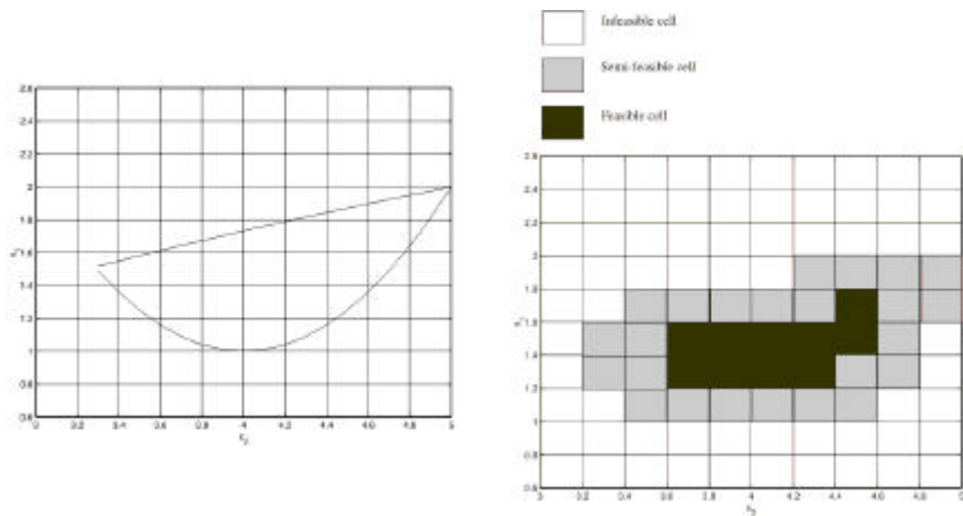
Figure 1: The figure at the left illustrates the feasible region of a problem. In this case, the lines represent the boundary between the feasible and infeasible regions. The figure at the right illustrates the representation of the constraints part of the belief space for the search space of the same problem.
